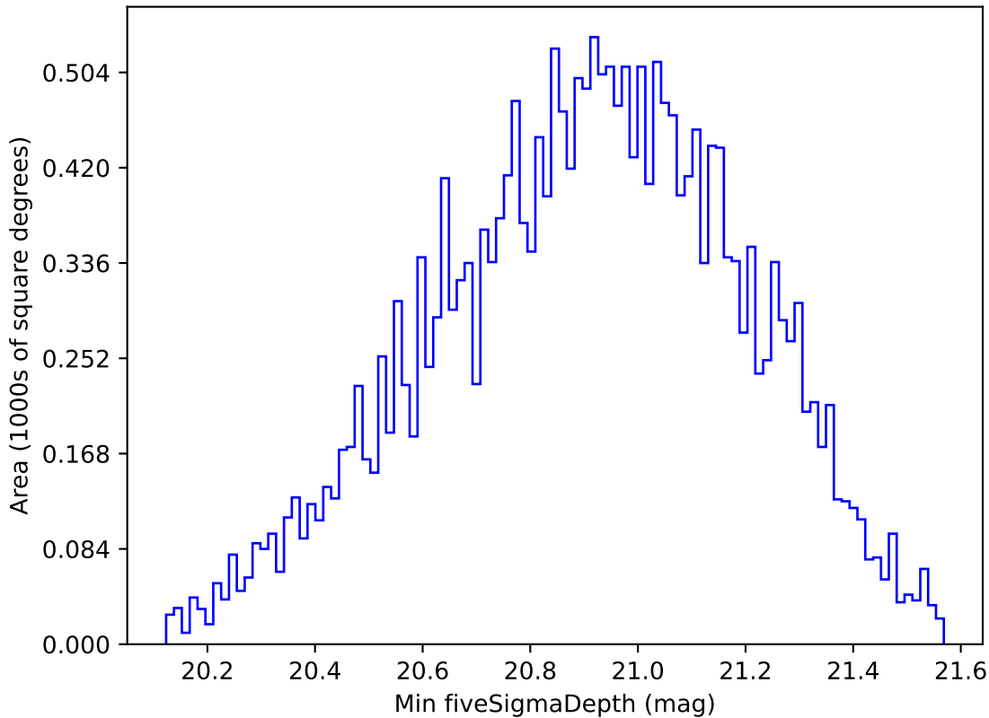
ddf_loaded_half_fl1_v3.4_10yrs All sky y band: Min fiveSigmaDepth
