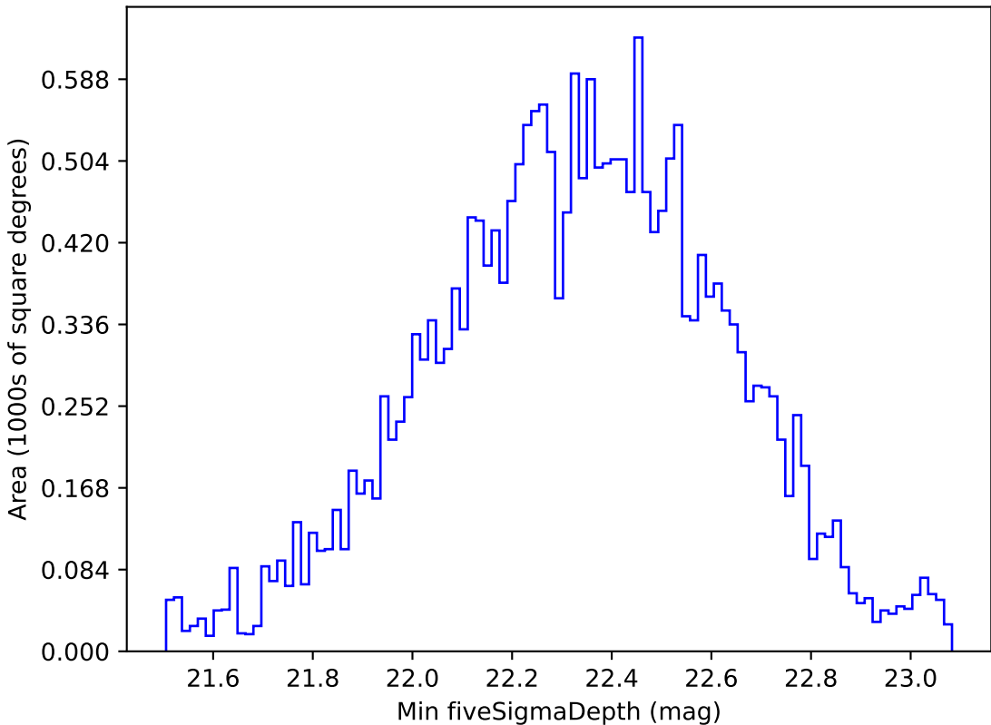
ddf_loaded_half_fl1_v3.4_10yrs All sky u band: Min fiveSigmaDepth
