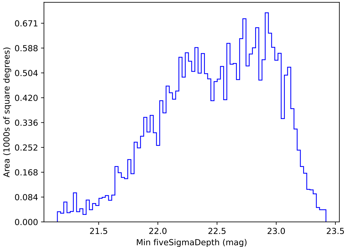
ddf_loaded_half_fl1_v3.4_10yrs All sky r band: Min fiveSigmaDepth
