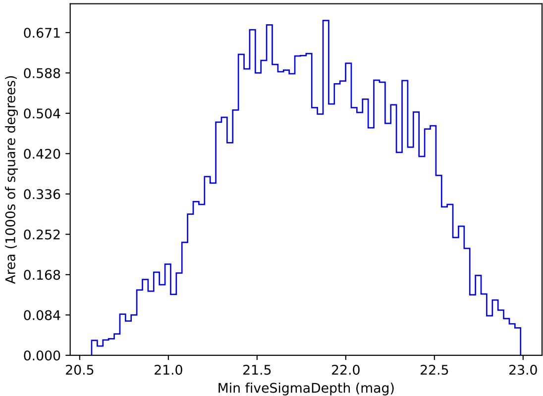
ddf_loaded_half_fl1_v3.4_10yrs All sky i band: Min fiveSigmaDepth
