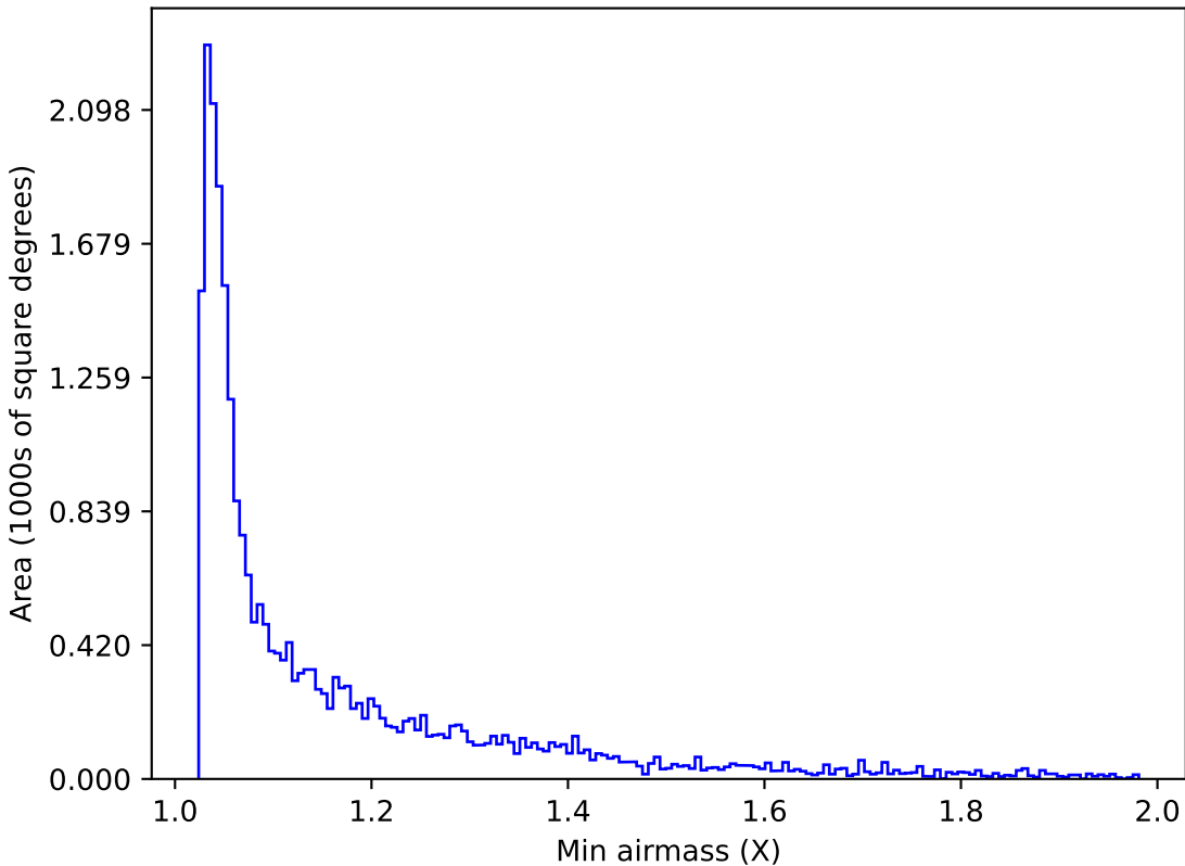
ddf_loaded_half_fl1_v3.4_10yrs Yr 1 z band: Min airmass
