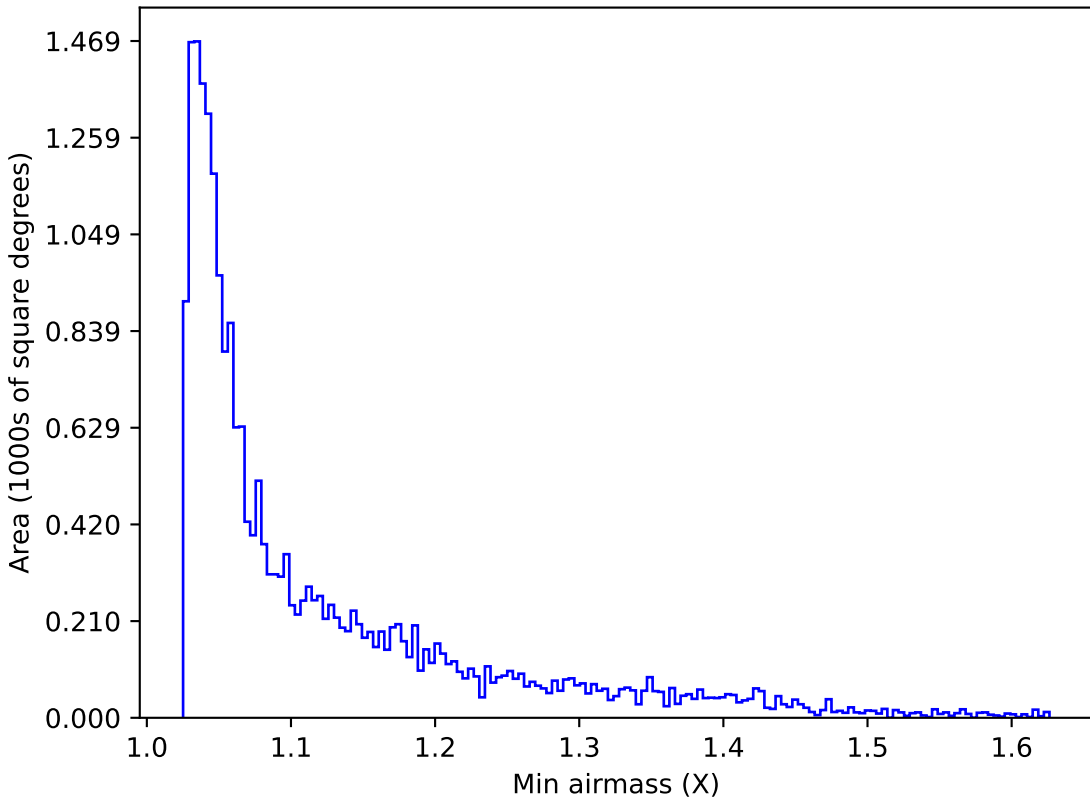
ddf_loaded_half_fl1_v3.4_10yrs Yr 1 y band: Min airmass
