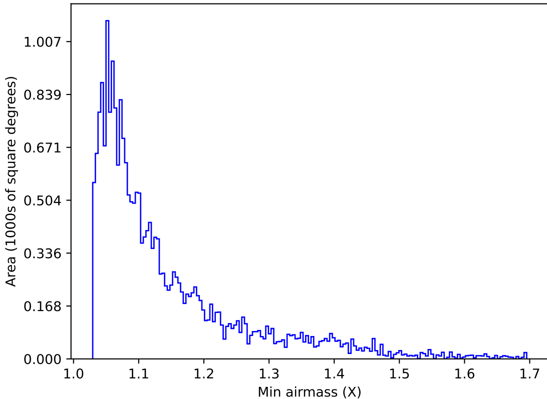
ddf_loaded_half_fl1_v3.4_10yrs Yr 1 u band: Min airmass
