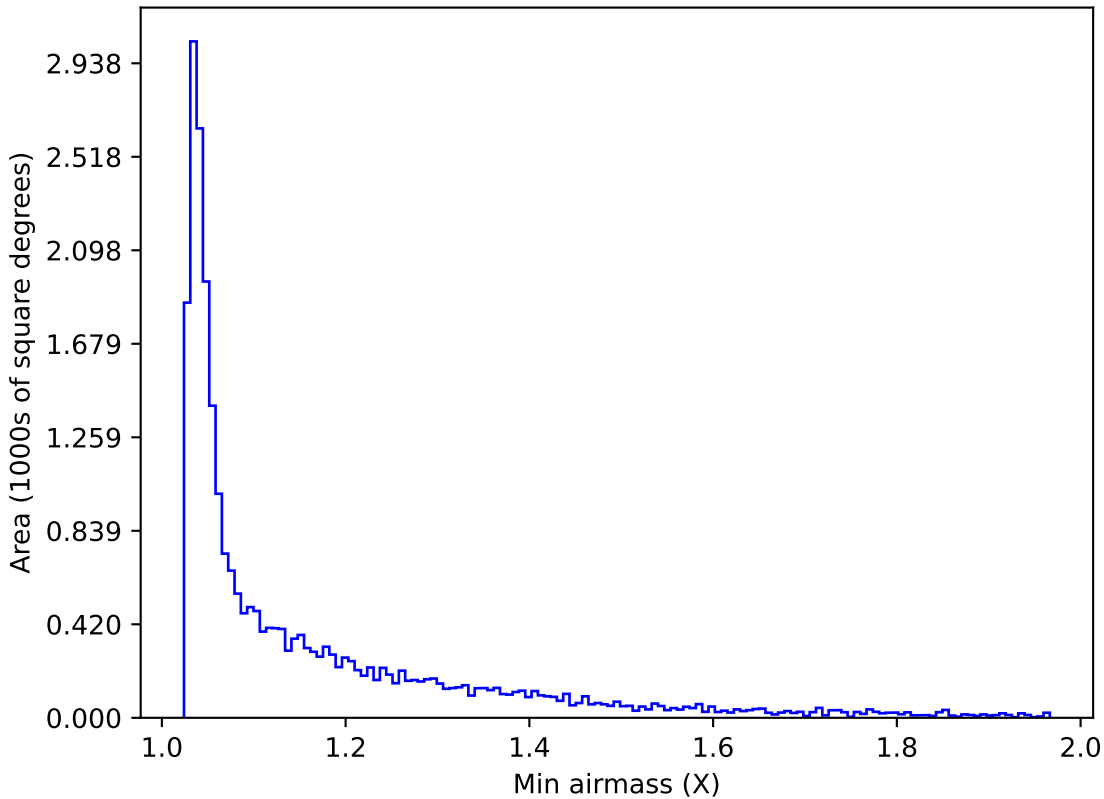
ddf_loaded_half_fl1_v3.4_10yrs Yr 1 r band: Min airmass
