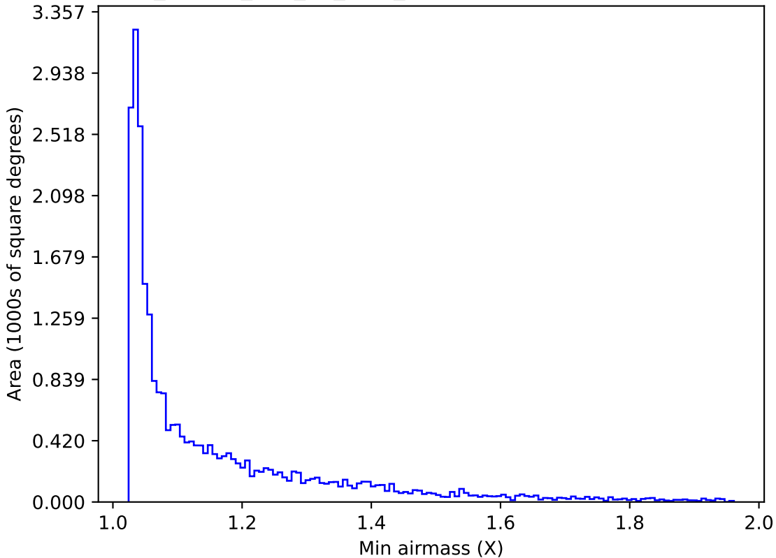
ddf_loaded_half_fl1_v3.4_10yrs Yr 1 i band: Min airmass
