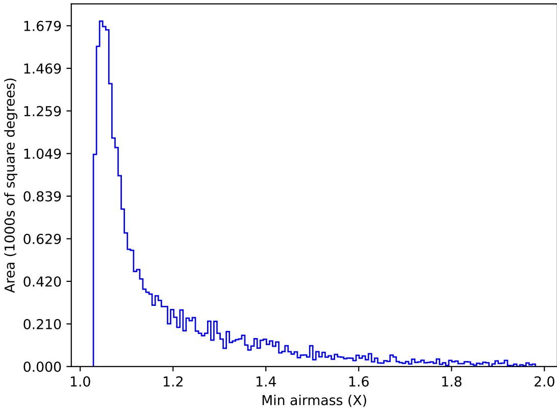
ddf_loaded_half_fl1_v3.4_10yrs Yr 1 g band: Min airmass
