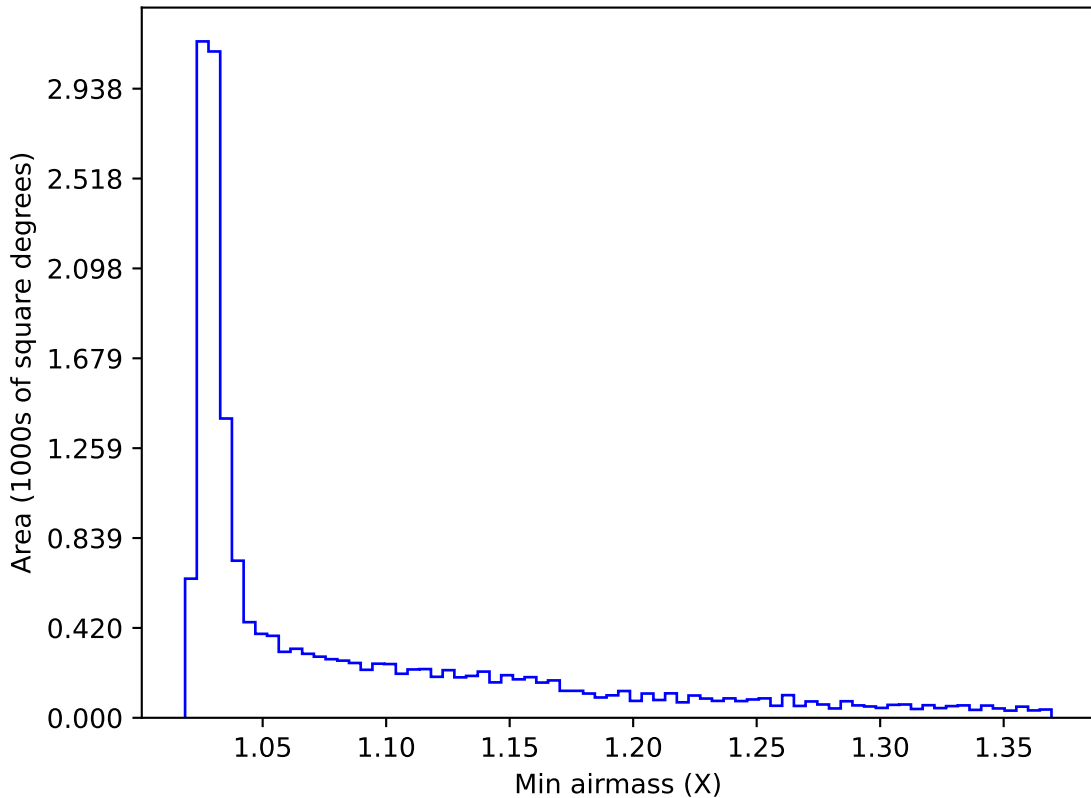
ddf_loaded_half_fl1_v3.4_10yrs WFD z band: Min airmass
