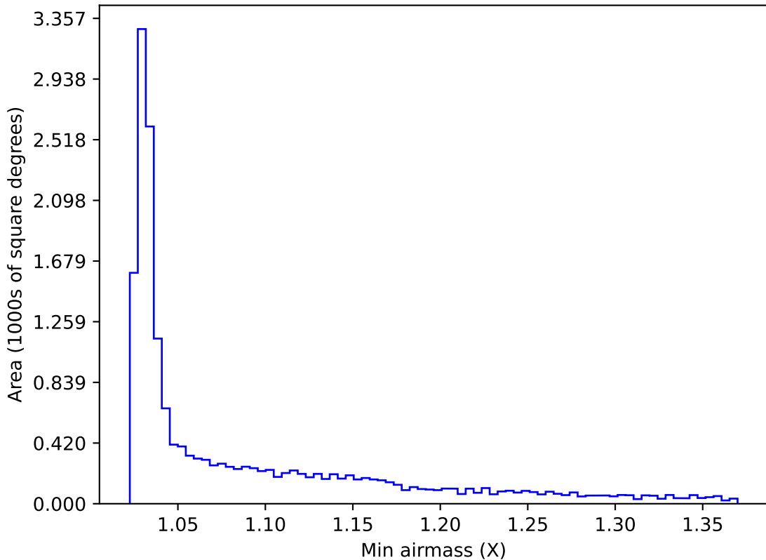
ddf_loaded_half_fl1_v3.4_10yrs WFD y band: Min airmass
