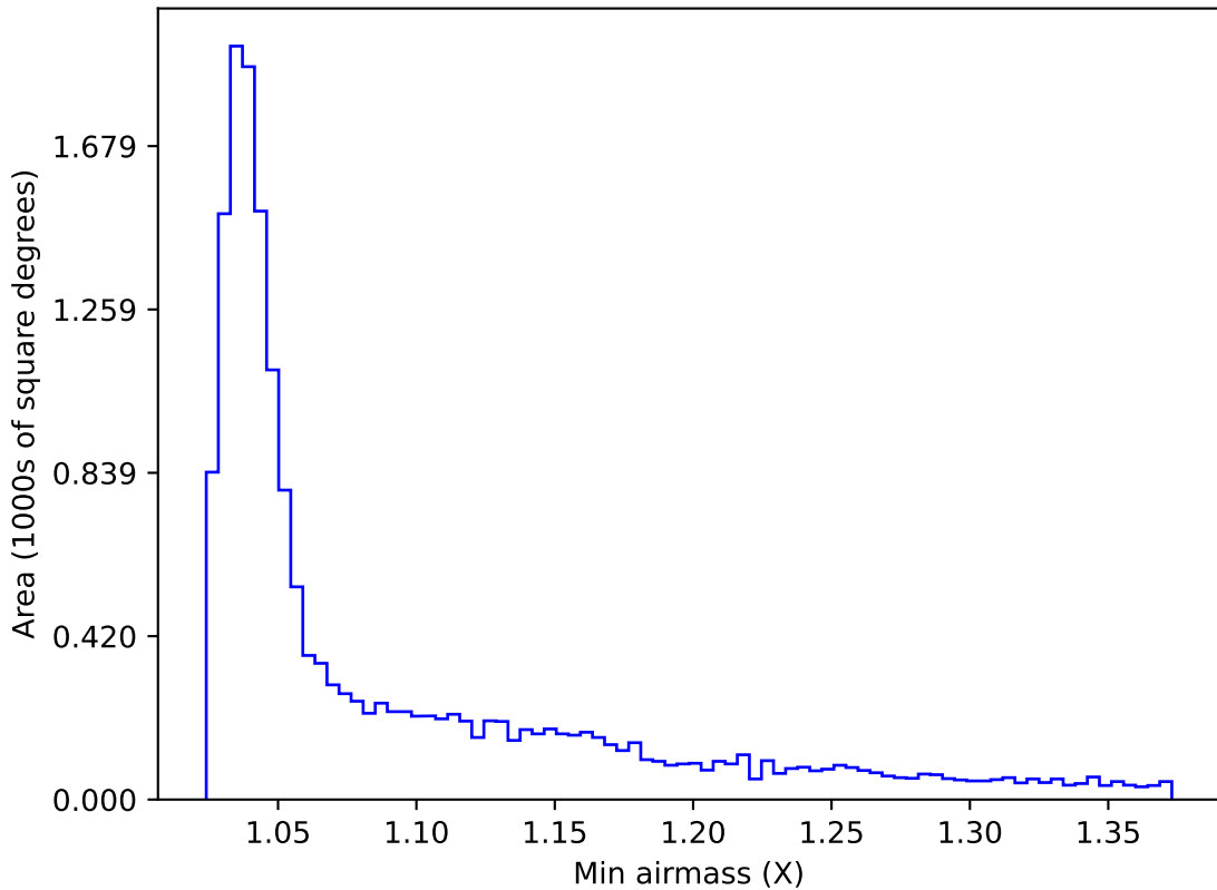
ddf_loaded_half_fl1_v3.4_10yrs WFD u band: Min airmass
