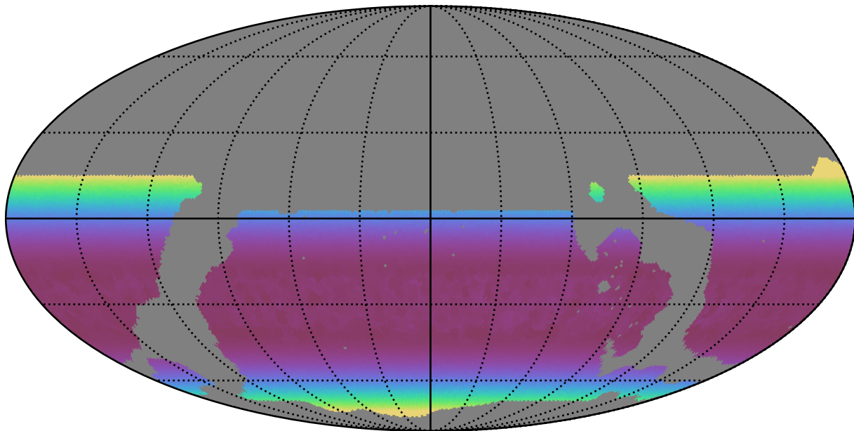
ddf_loaded_half_fl1_v3.4_10yrs WFD r band: Min airmass
