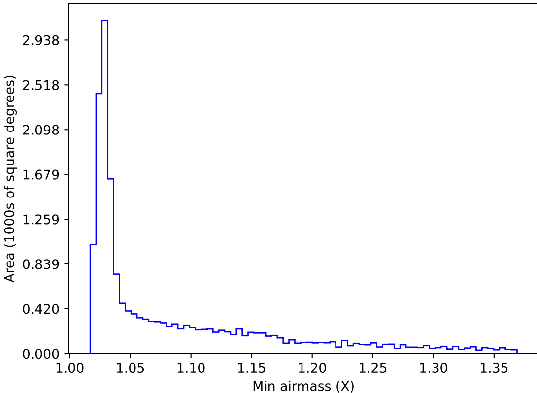
ddf_loaded_half_fl1_v3.4_10yrs WFD r band: Min airmass
