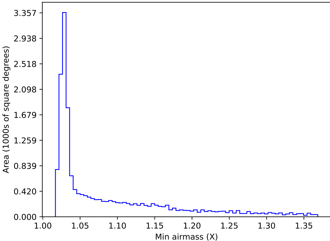
ddf_loaded_half_fl1_v3.4_10yrs WFD i band: Min airmass
