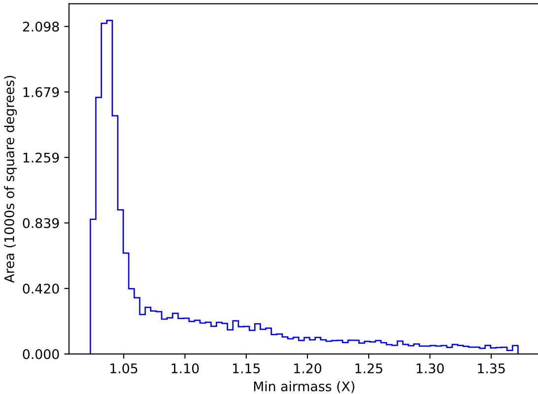
ddf_loaded_half_fl1_v3.4_10yrs WFD g band: Min airmass
