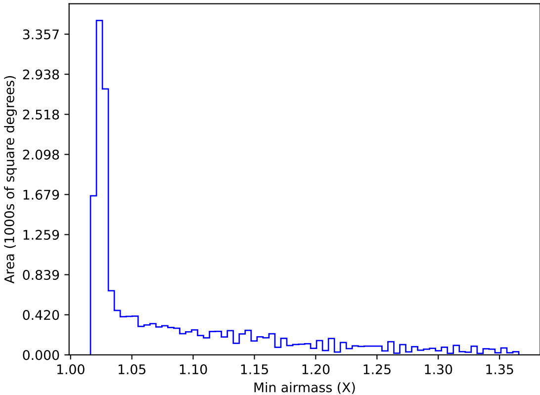
ddf_loaded_half_fl1_v3.4_10yrs WFD all bands: Min airmass
