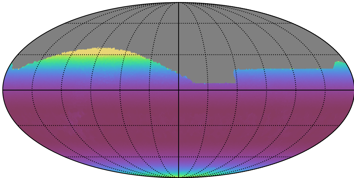
ddf_loaded_half_fl1_v3.4_10yrs All sky z band: Min airmass
