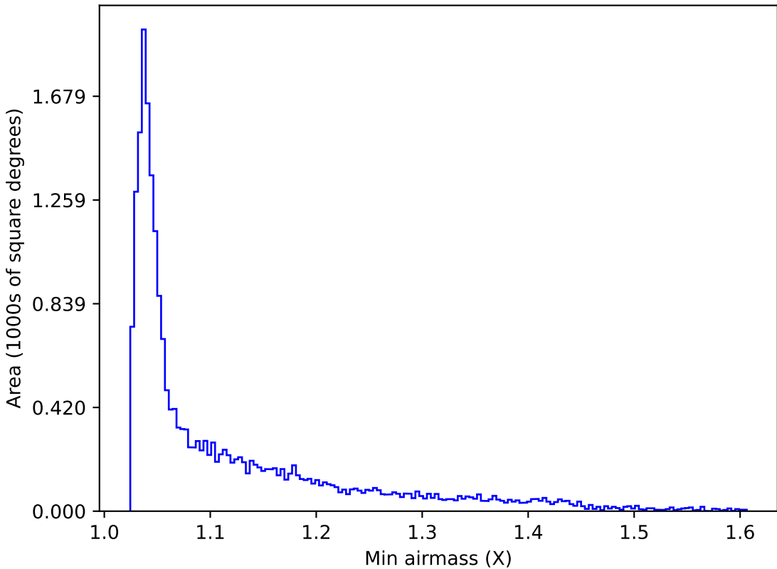
ddf_loaded_half_fl1_v3.4_10yrs All sky u band: Min airmass
