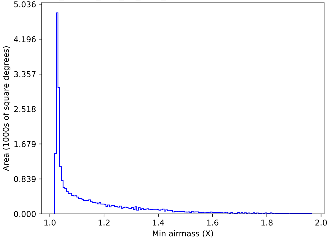
ddf_loaded_half_fl1_v3.4_10yrs All sky i band: Min airmass
