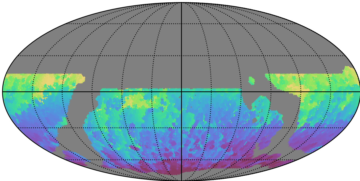
ddf_loaded_half_fl1_v3.4_10yrs WFD z band: Min HA
