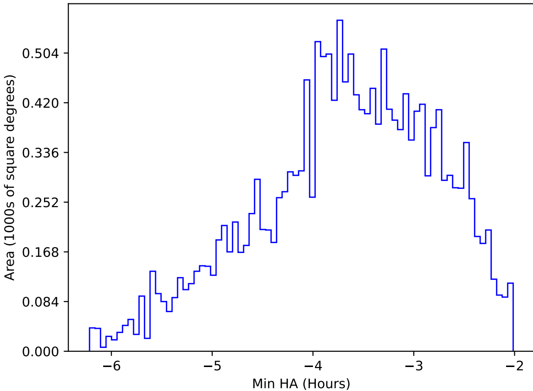
ddf_loaded_half_fl1_v3.4_10yrs WFD y band: Min HA
