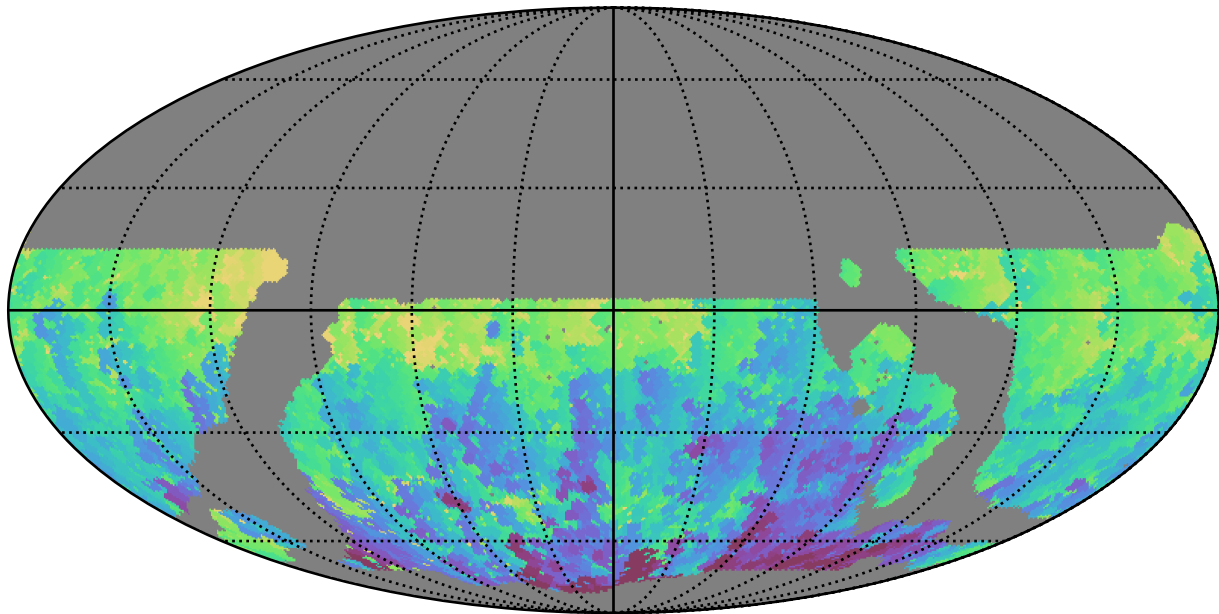
ddf_loaded_half_f11_v3.4_10yrs WFD u band: Min HA
