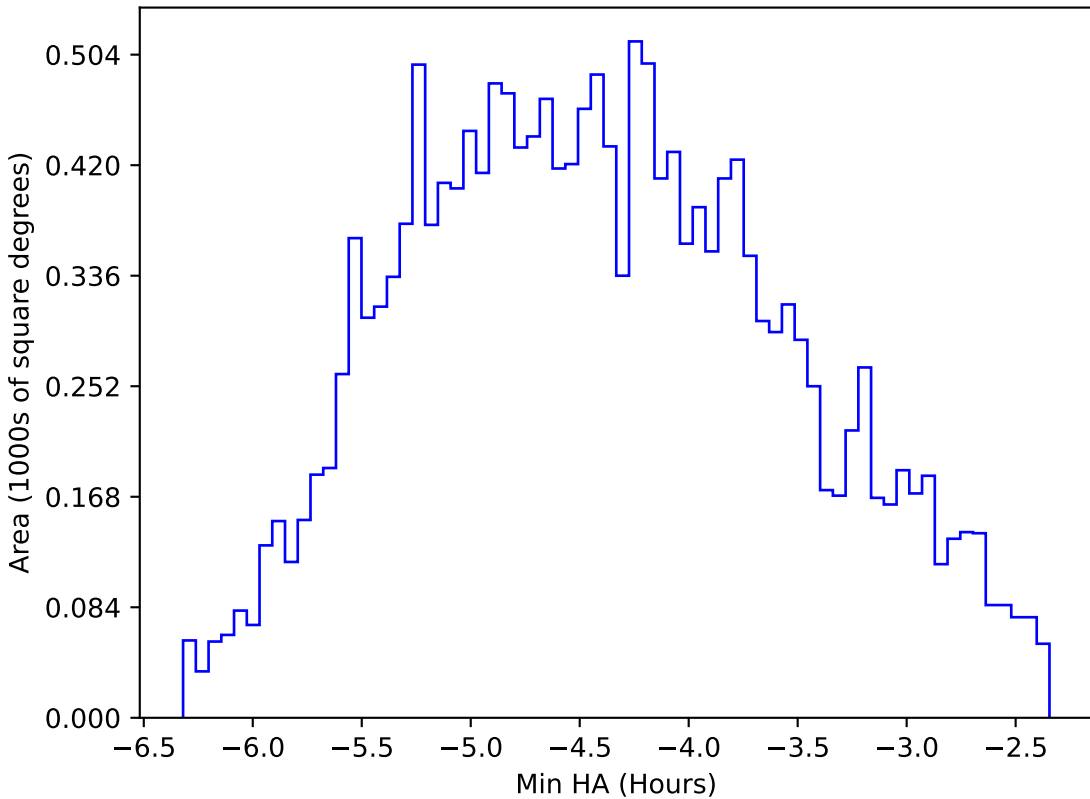
ddf_loaded_half_fl1_v3.4_10yrs WFD r band: Min HA
