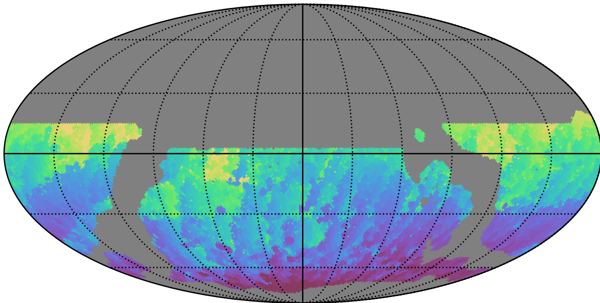
ddf_loaded_half_fl1_v3.4_10yrs WFD i band: Min HA
