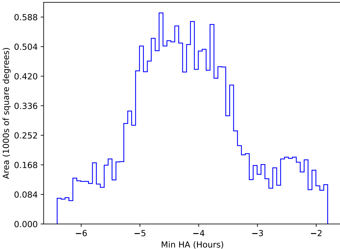
ddf_loaded_half_fl1_v3.4_10yrs WFD g band: Min HA
