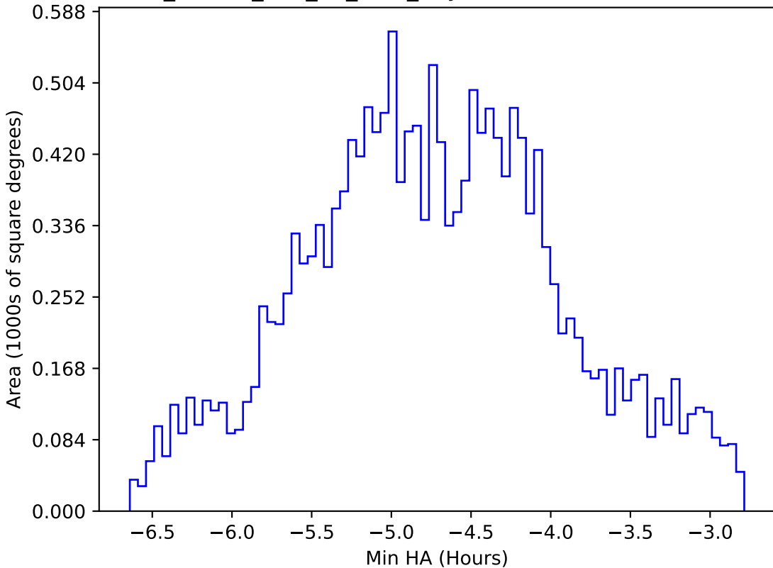
ddf_loaded_half_fl1_v3.4_10yrs WFD all bands: Min HA
