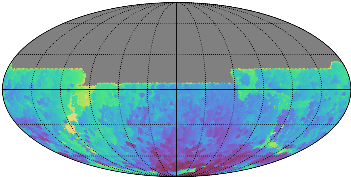
ddf_loaded_half_f11_v3.4_10yrs All sky y band: Min HA
