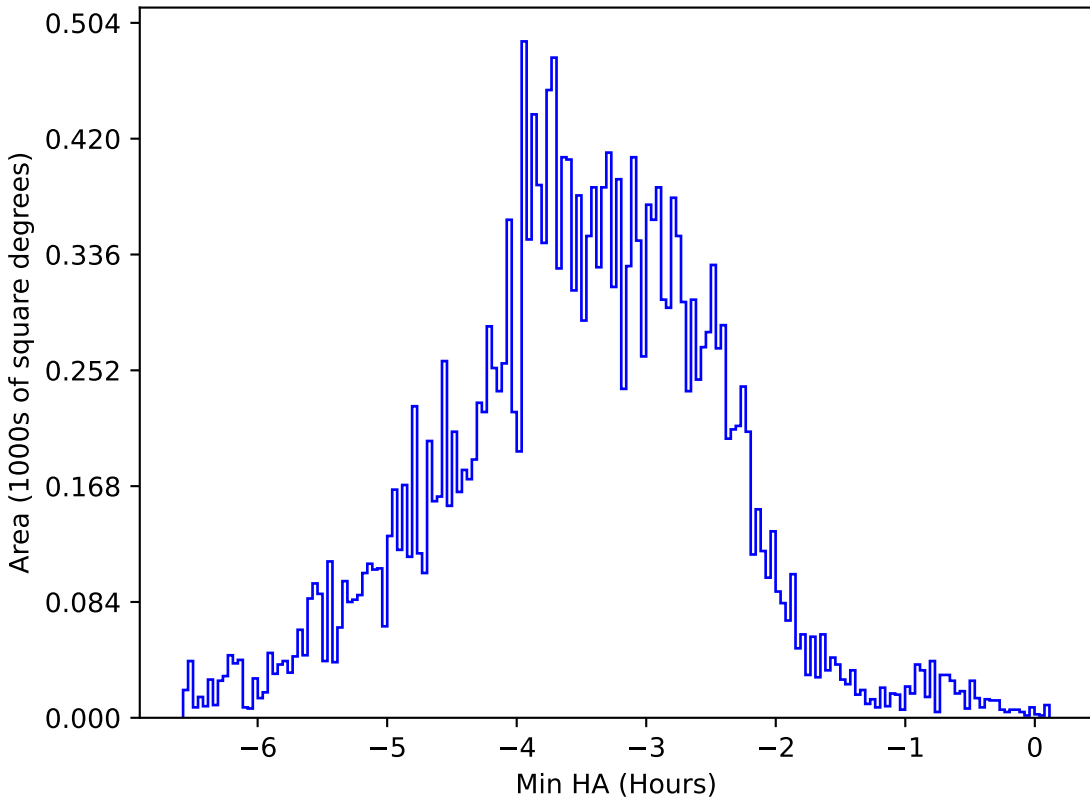
ddf_loaded_half_fl1_v3.4_10yrs All sky y band: Min HA
