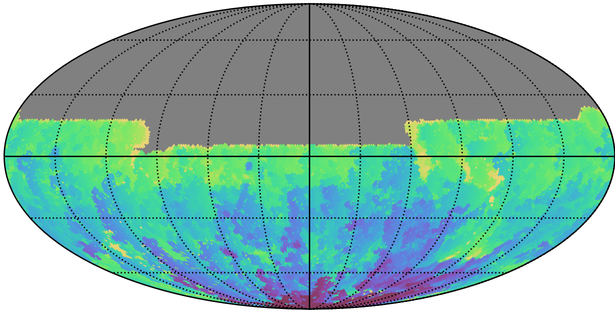
ddf_loaded_half_f11_v3.4_10yrs All sky u band: Min HA
