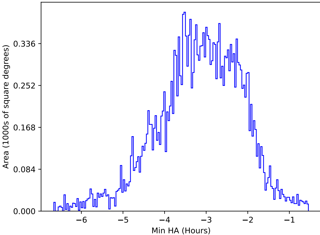
ddf_loaded_half_fl1_v3.4_10yrs All sky u band: Min HA
