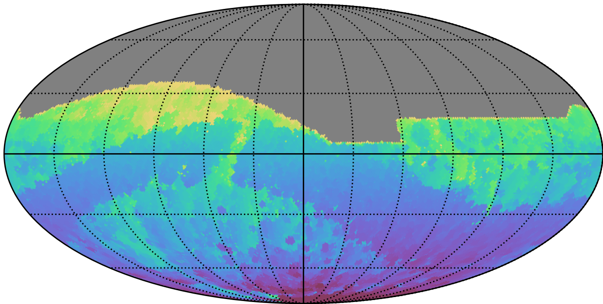
ddf_loaded_half_fl1_v3.4_10yrs All sky r band: Min HA
