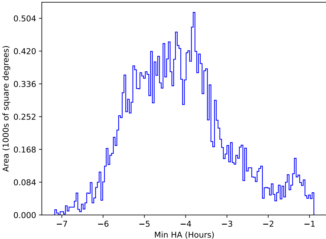
ddf_loaded_half_fl1_v3.4_10yrs All sky r band: Min HA
