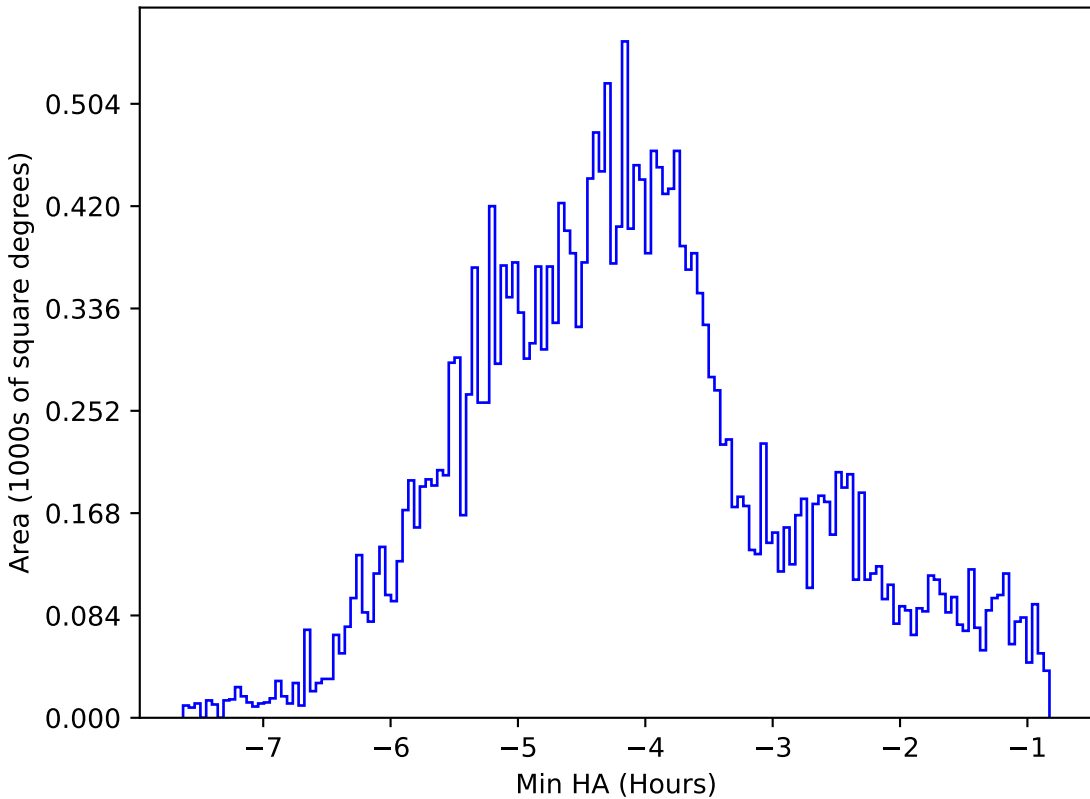
ddf_loaded_half_fl1_v3.4_10yrs All sky i band: Min HA
