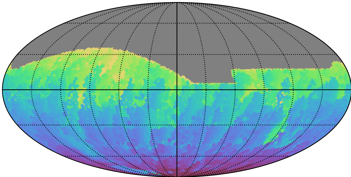
ddf_loaded_half_f11_v3.4_10yrs All sky g band: Min HA
