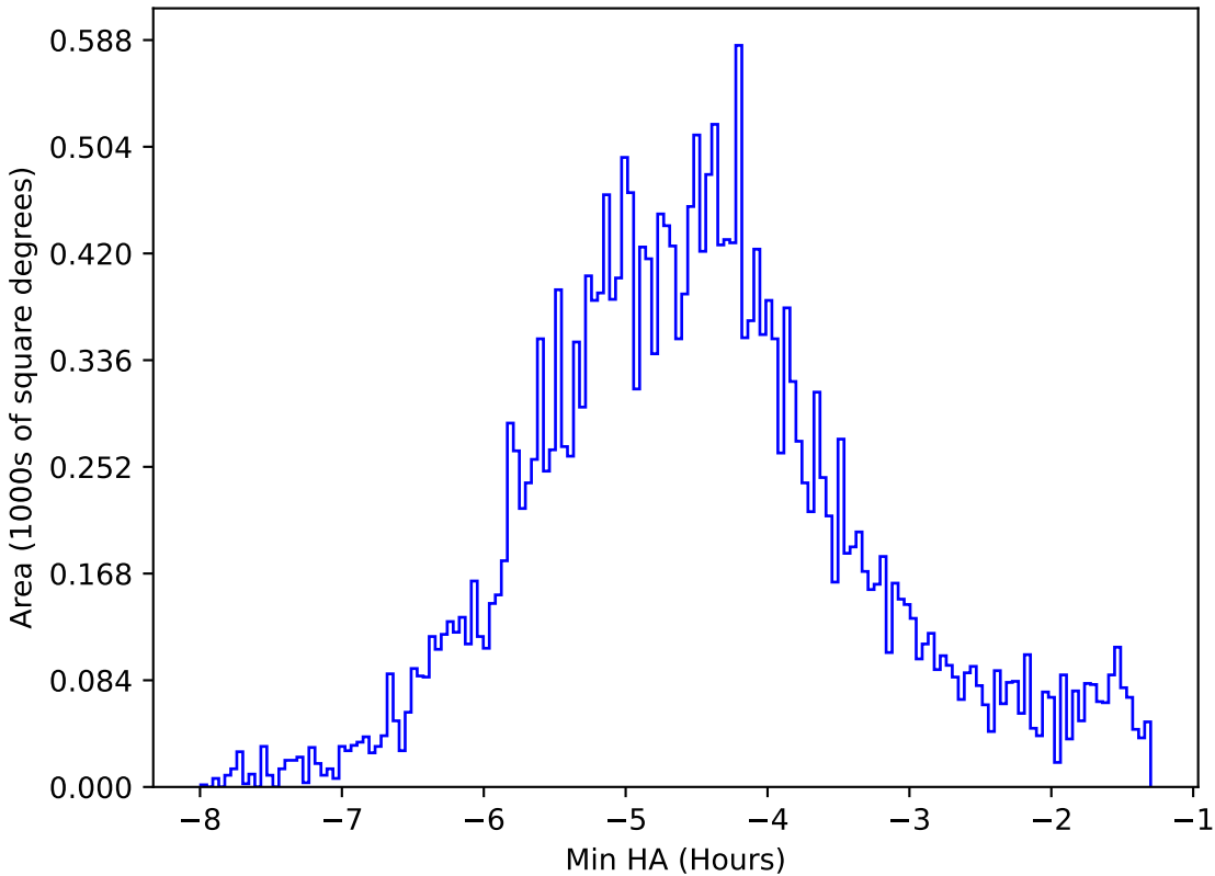
ddf_loaded_half_fl1_v3.4_10yrs All sky all bands: Min HA
