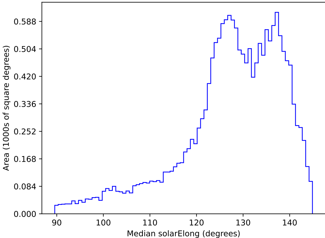
ddf_loaded_half_fl1_v3.4_10yrs WFD z band: Median solarElong
