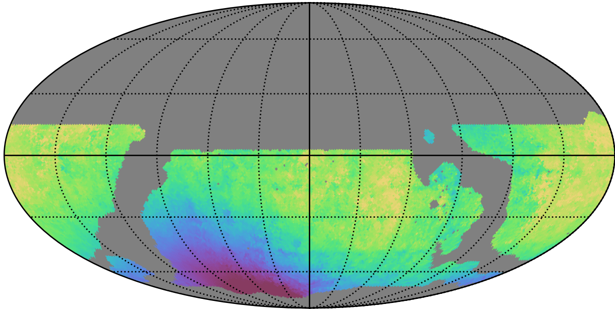
ddf_loaded_half_fl1_v3.4_10yrs WFD y band: Median solarElong
