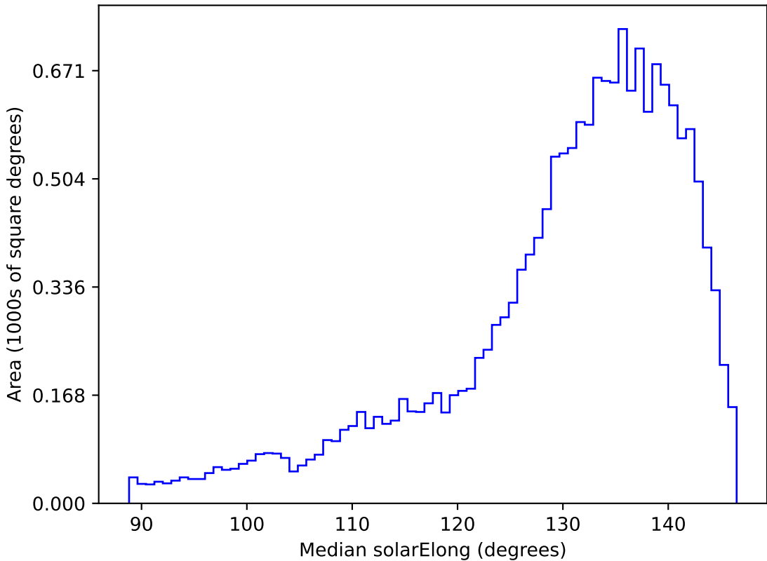
ddf_loaded_half_fl1_v3.4_10yrs WFD y band: Median solarElong
