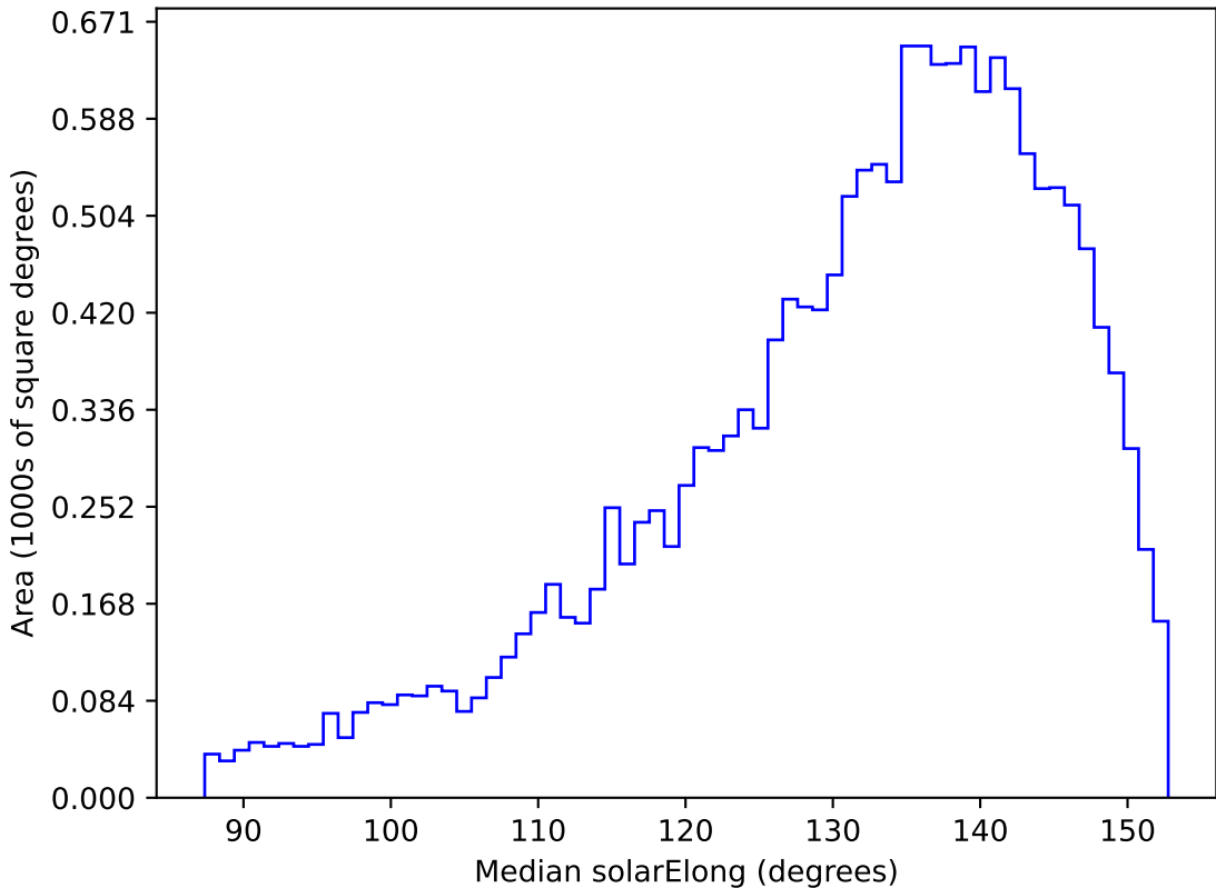
ddf_loaded_half_fl1_v3.4_10yrs WFD u band: Median solarElong
