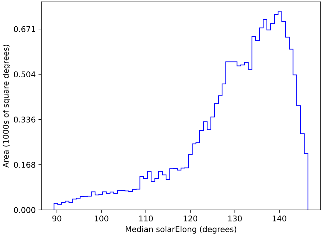
ddf_loaded_half_fl1_v3.4_10yrs WFD r band: Median solarElong
