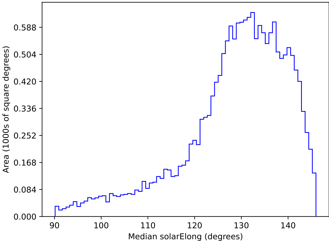
ddf_loaded_half_fl1_v3.4_10yrs WFD i band: Median solarElong
