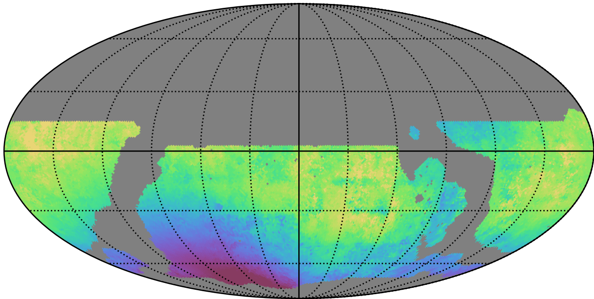
ddf_loaded_half_fl1_v3.4_10yrs WFD g band: Median solarElong
