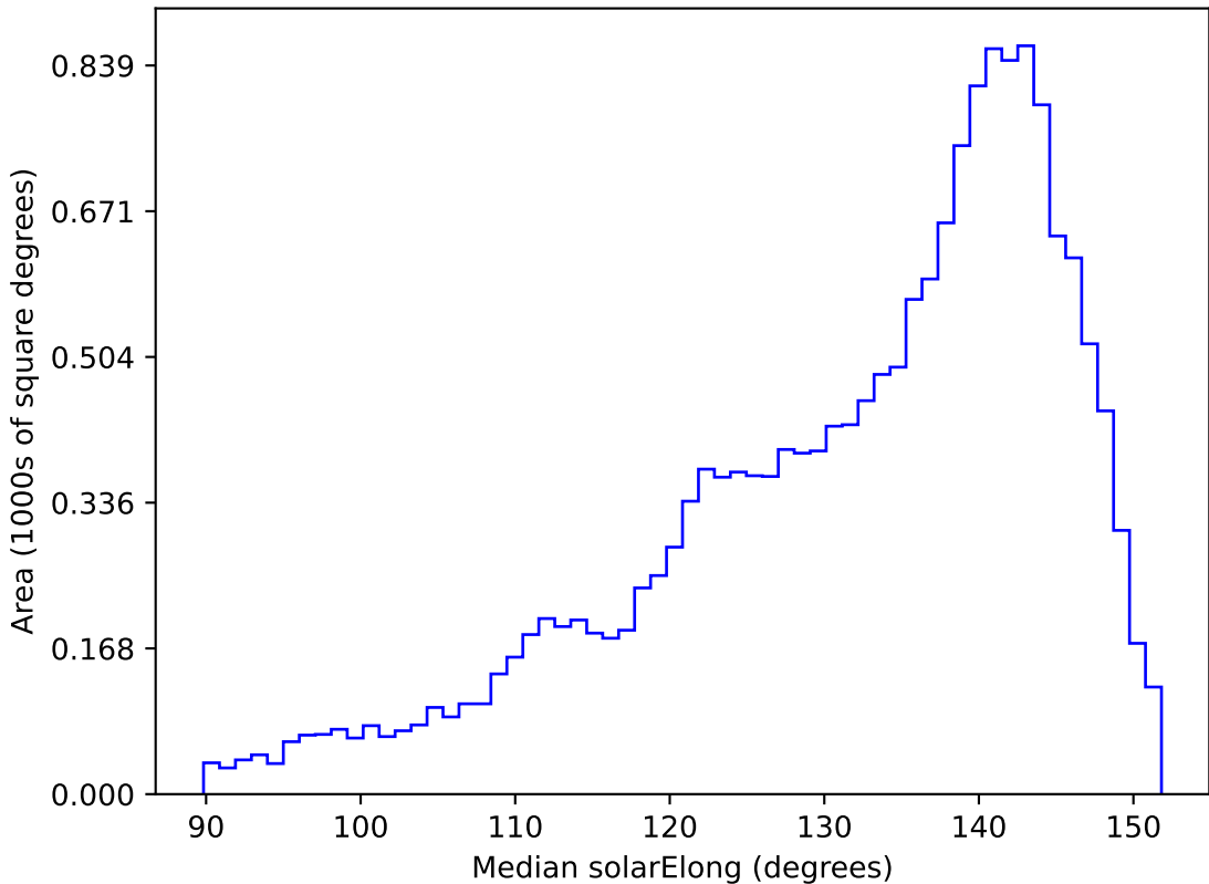
ddf_loaded_half_fl1_v3.4_10yrs WFD g band: Median solarElong
