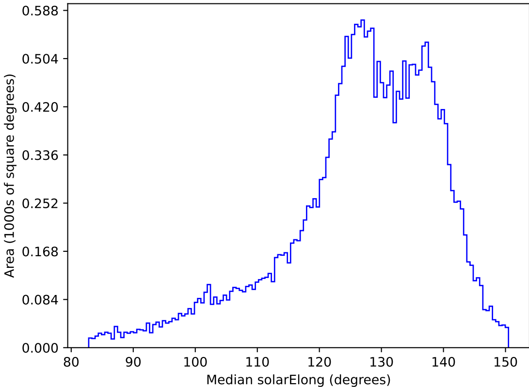
ddf_loaded_half_fl1_v3.4_10yrs All sky z band: Median solarElong
