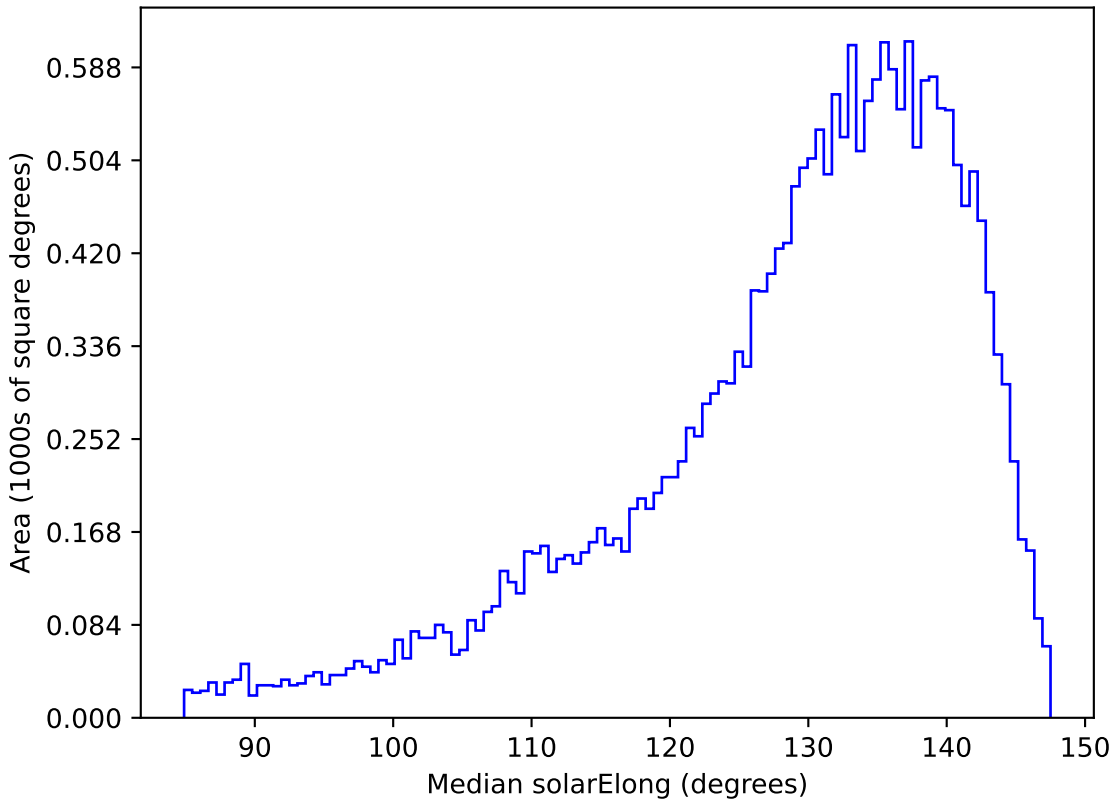
ddf_loaded_half_fl1_v3.4_10yrs All sky y band: Median solarElong
