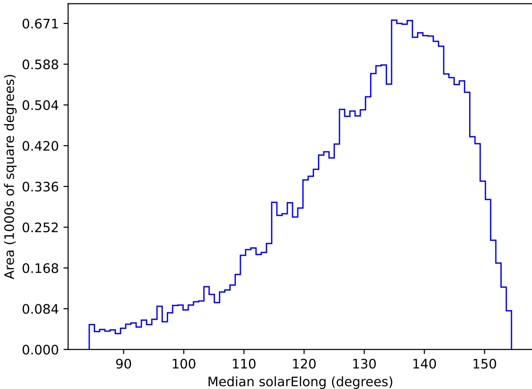
ddf_loaded_half_fl1_v3.4_10yrs All sky u band: Median solarElong
