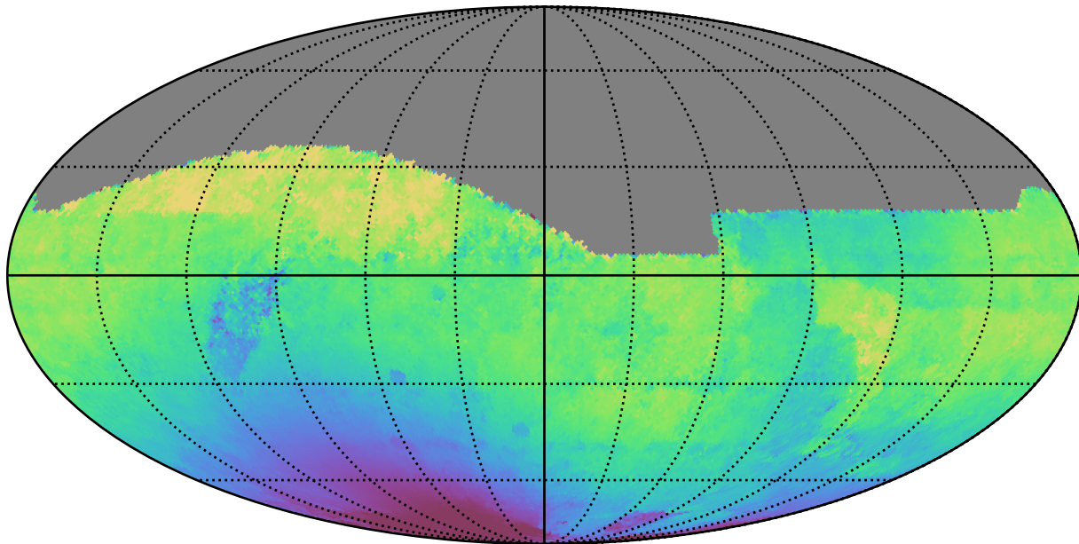
ddf_loaded_half_fl1_v3.4_10yrs All sky r band: Median solarElong
