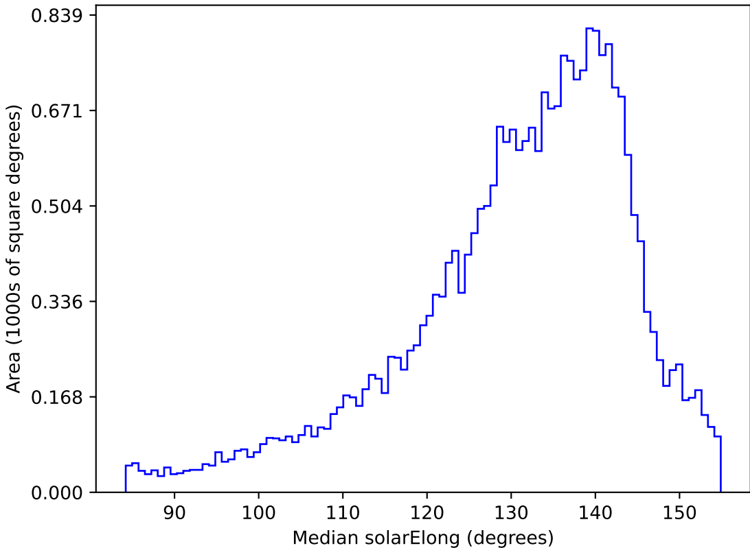
ddf_loaded_half_fl1_v3.4_10yrs All sky r band: Median solarElong
